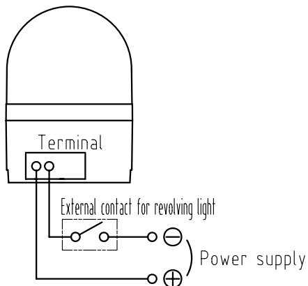
Wiring example
