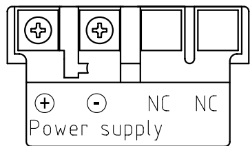
Terminal view
