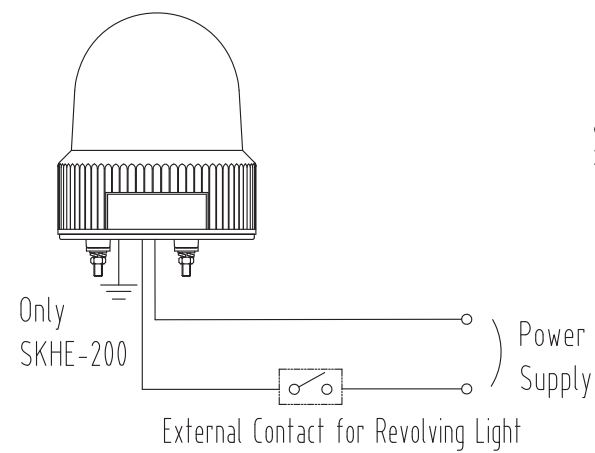
Wiring Example
